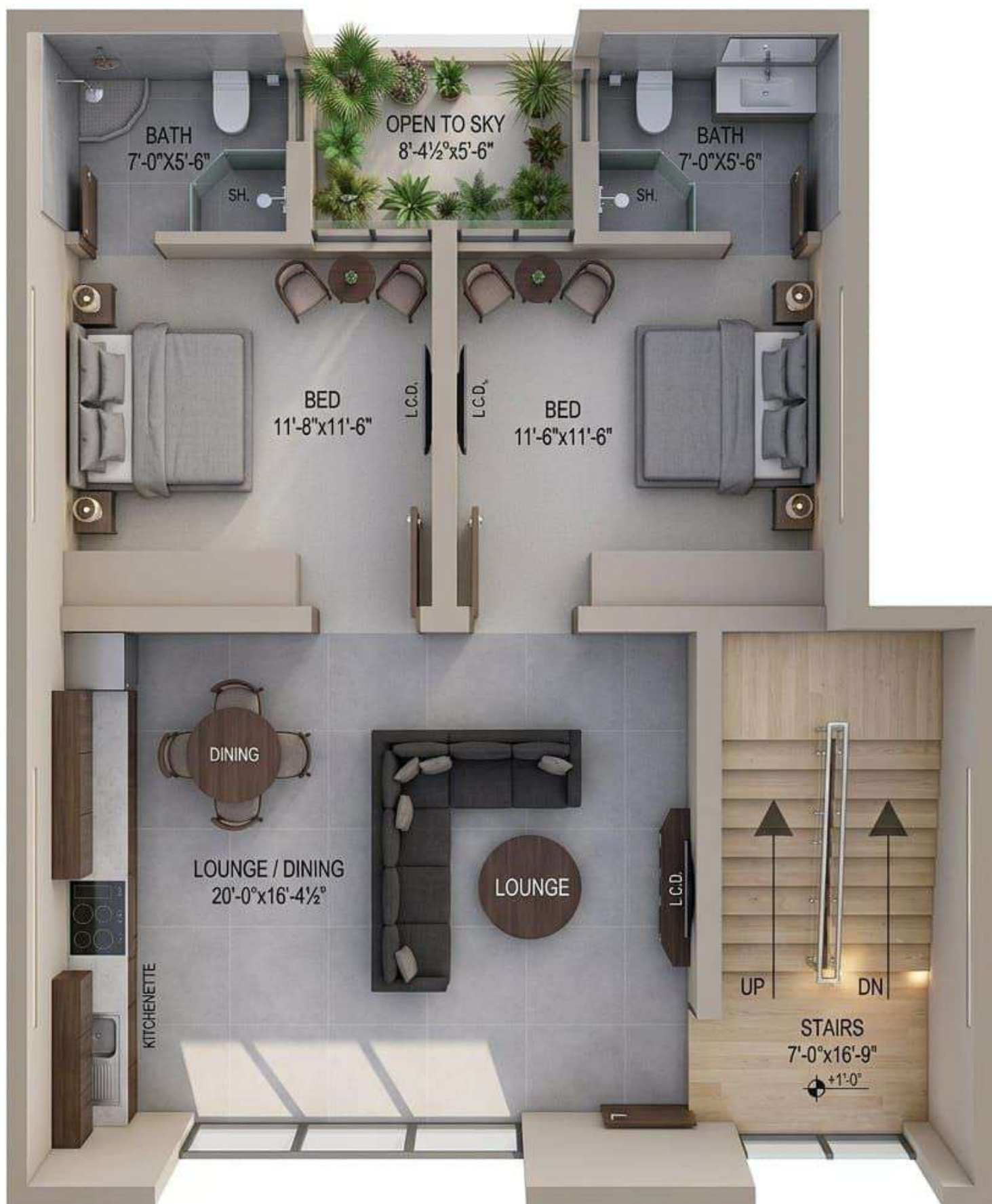
5 MARLA MODULE -01 SIZE 25'-0"x45'-0" SECOND FLOOR
